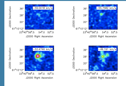
Figure 2: (generated using the CASA Viewer) Channel maps of 3.28 km s -1 resolution CARMA HCO + data.
