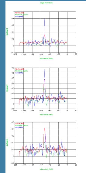
Figure 3: (from the CASA Viewer) CARMA HCO + , CS, & CH 3 OH spectra at: blue-shifted outflow peak (upper); continuum peak (middle); and red-shifted outflow peak (lower)
