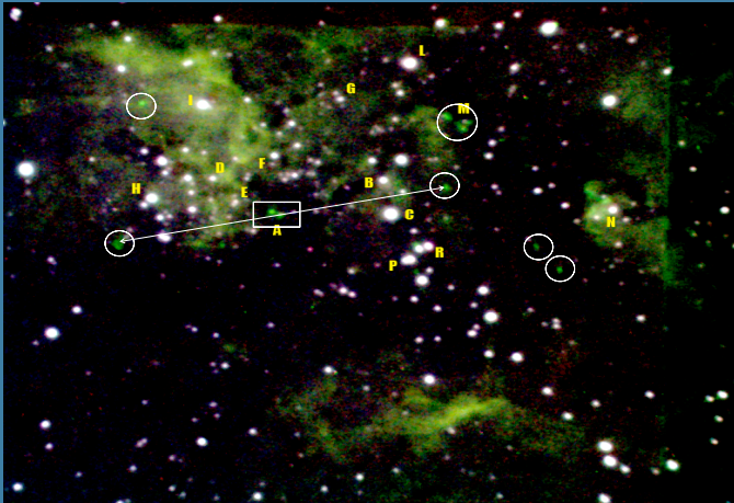
Figure 1a: Mol 160 region (IRAS 23385+6053): Combined H 2 2.12 μm (green), H 2 -continuum 2.13 μm (blue), and H 2 2.25 μm (red) images. YSOs (letters) with 24 μm detections identified in Table 1 of Molinari et al. (2008) are indicated. The box indicates the pull-out in Fig. 1b of Mol 160 A, which is a confirmed massive protostar. Note the bright bipolar H 2 2.12 μm knots associated with this object and the complete lack of continuum emission. Other identified MHOs are circled. The double arrow links two MHOs that are aligned along the direction of the large-scale CO outflow identified by Zhang et al. (2005).
