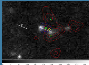
Figure 1b: Mol 160 A - MHOs (greyscale) CS & 3 mm continuum core peak (diamond) Class I CH 3 OH masers (x) HCO + outflow (blue & red contours) (from 0.55 km s -1 resolution data) Blue: -57.3945 to -54.1115 km s -1 Red: -50.8285 to -47.5455 km s -1
